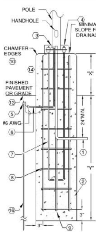
SECTION VIEW
